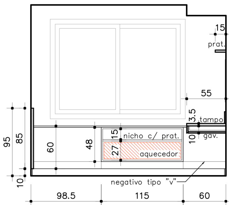
PAINEL - VISTA
